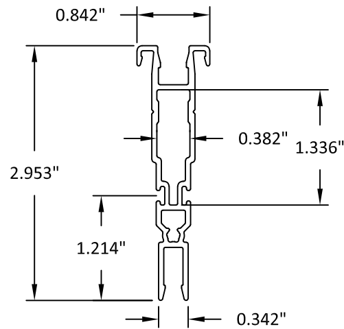
MULLION DETAIL
